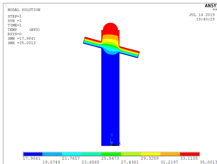
Fig. 6. Temperature fields in the cross section of LED SOLAR SPOT® D.530 hybrid HTLG. The model is divided into 2704121 elements
