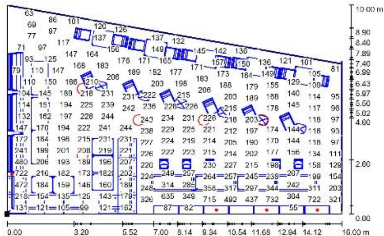
Fig. 5. Table of illumination values in the airport terminal cafe. Work plane. Graph of values of E (E average value = 194 Lx; Emin = 27 Lx; Emax = 1007 Lx; Emin / E average value = 0.137; Emin / Emax = 0.026. Scale 1: 115. Developed in improved DIALux program
