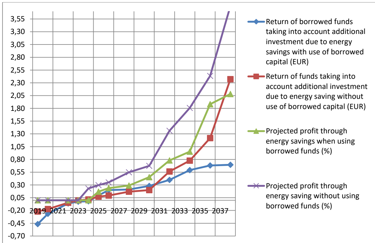
Fig. 8. Calculation of the dynamics of funds return with additional investment to the project due to energy savings associated with use of energy-efficient daylighting hybrid systems LEDSOLARSPOT® D.530, along the ordinate axis - euro
