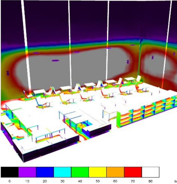
Fig. 4. The illumination scheme of the terminal building cafe using Bell/T LED 50v D15 4000K lamps (5 pcs.) and LEDSOLARSPOT® D.530 hybrid HTLG (5 pcs.). Dummy colors - visualization. Performed in improved DIALux program
