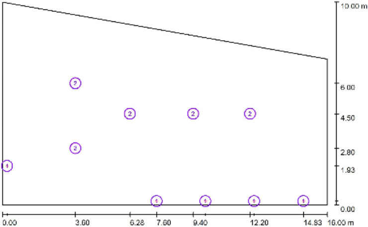
Fig. 3. The layout of the fixtures (No. 1 - Bell / T LED 50v D15 4000K, No. 2 - Solarspot® D.530, scale 1: 115). Performed in the improved DIALux program
