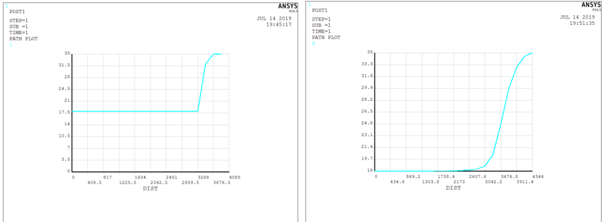
Fig. 7. Temperature distribution graphs: - along the Z axis of LEDSOLARSPOT® D.530 HTLG (X coordinate = 316 mm, Y = 0 mm) - to the left; - along the Z axis of LEDSOLARSPOT® D.530 HTLG (coordinate X = 0 mm, Y = 0 mm) - to the right.
